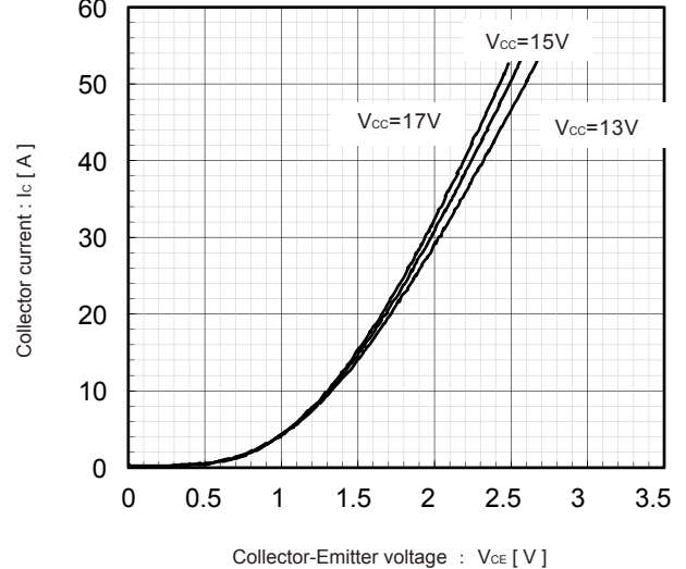
Collector current vs. Collector-Emittter voltage T_j=125^\circ\text{C} [Terminal] (typ.)
