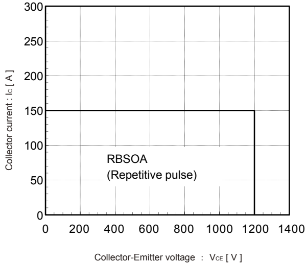
Reversed biased safe operating area V_{ce}=15V, T_J \le 125^\circ C
