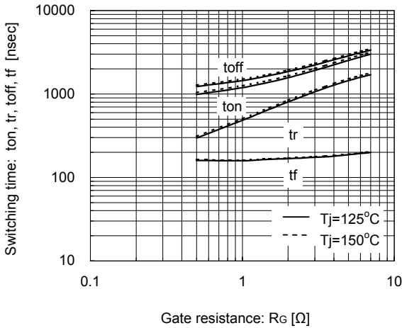
[INVERTER]
