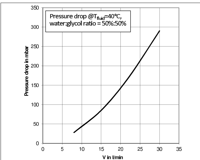
Fig. 10: Pressure drop \Delta p versus flow rate V
