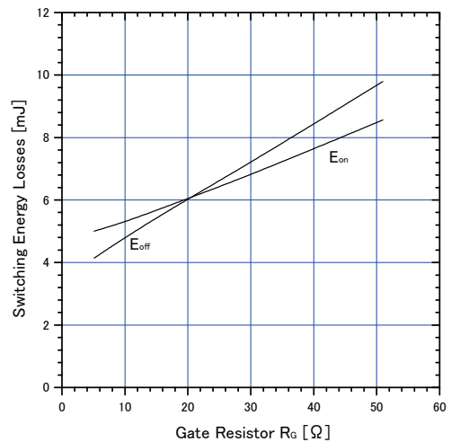
Graph.12 Typical switching losses vs. RG T_j=175^\circ C, V_{CC}=600V, I_c=75A, L=500\mu H V_{GE}=15V
