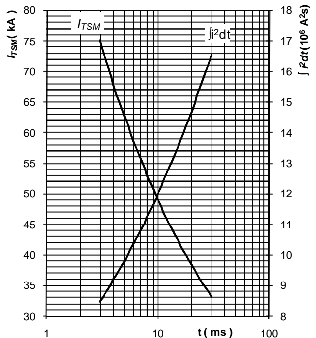
Fig. 4 Surge on-state current vs. pulse length, half sine wave, single pulse, V_R = 0 V, T_j = T_{jmax}
