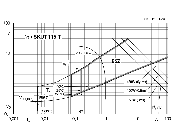
Fig. 10: Gate trigger characteristic
